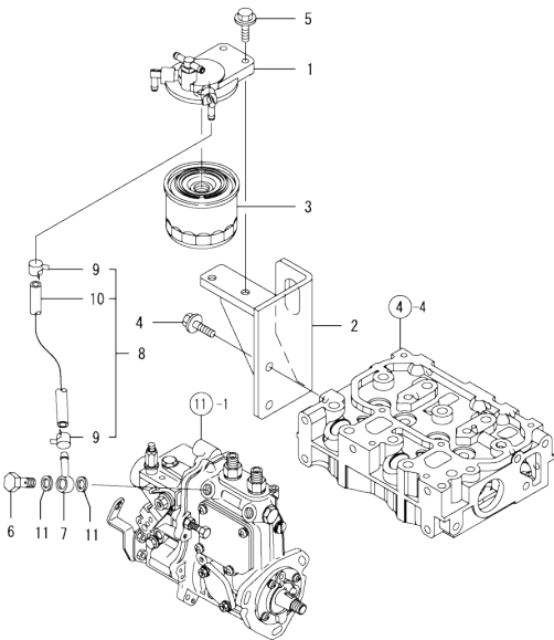
Fig.14. FUEL LINE
