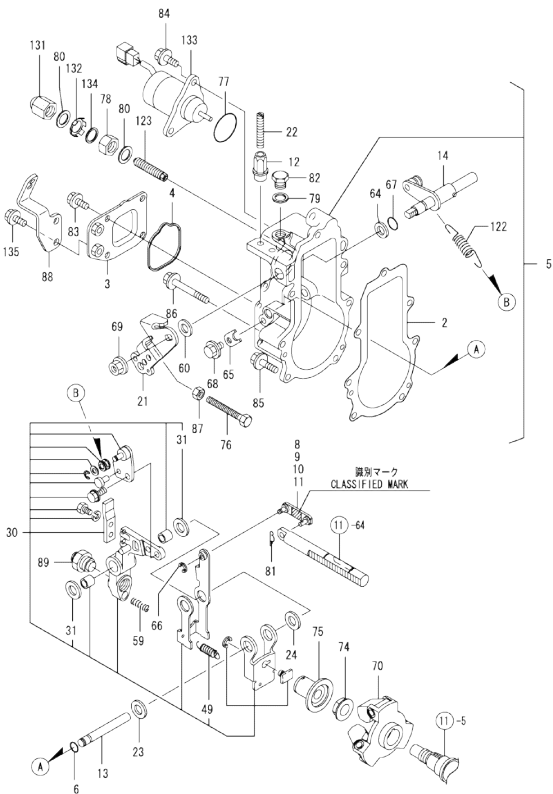
Fig.12. GOVERNOR
